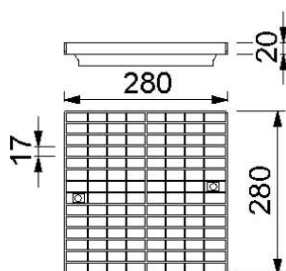
Galvanized mesh grating 20/30, B 125
