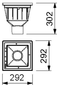
MEAPARK Yard Gully
