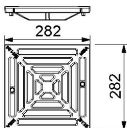
Ductile iron grating, B 125
